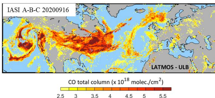
CO total columns from IASI as tracers of cross Atlantic transport of Californian fires
