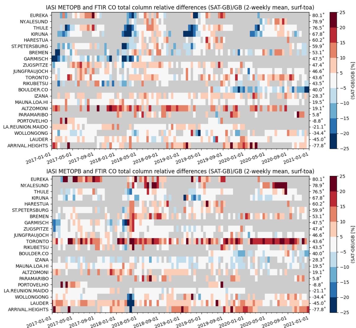
Figure 2.6. Time series of bi-weekly relative difference for IASI Metop-B against NDACC FTIR for the direct comparison (top) and the comparison with smoothing (bottom).
