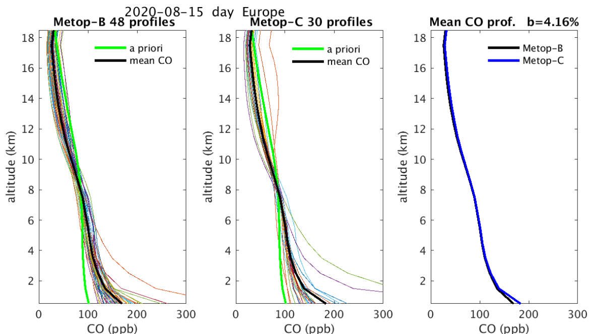
Figure 3.10. Same as Figs 3.6 to 3.9 but for 2020-08-15, over the European region.
