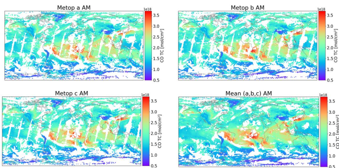
Figure 3.1. 1x1 degree median grids of IASI-A, B, and C daytime observations of October 7 2019, taken as an example. The last panel is the mean of the three Metops.
