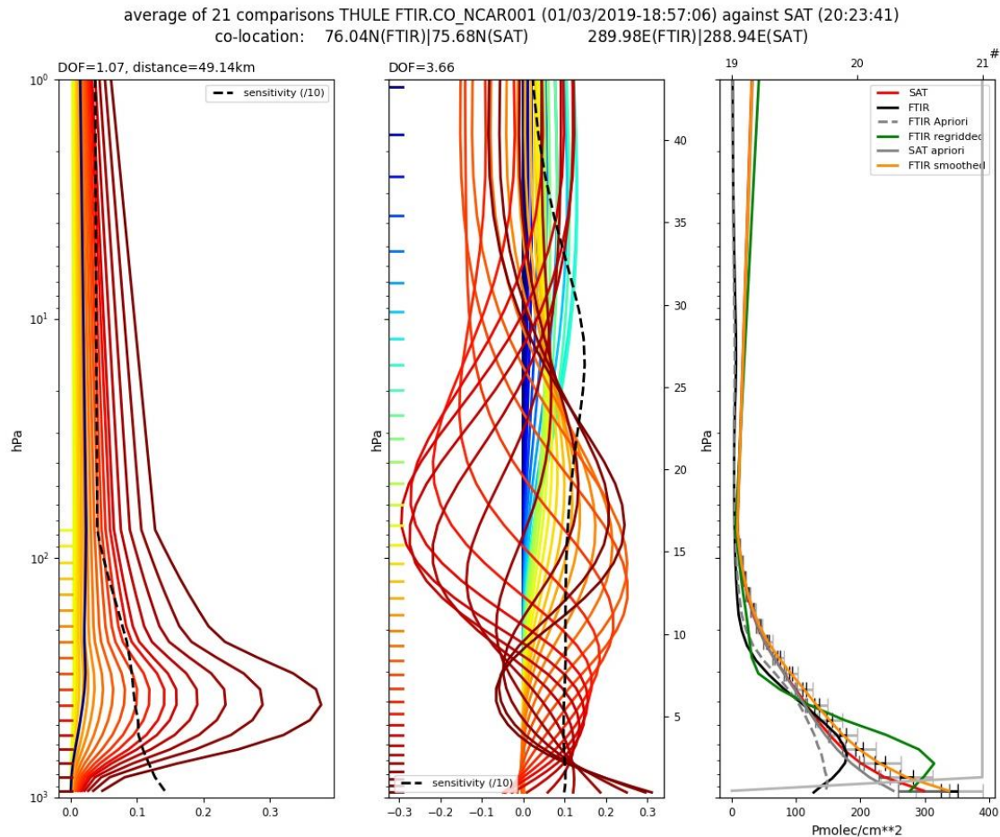
Figure 2.3. A detailed profile comparison plot for a single FTIR measurement against the average of 21 co-located IASI Metop-B retrieved profiles during spring 2019 at Thule (Greenland). The plot consists of 3 panels: the IASI AVK acting on partial column profiles (left), the FTIR AVK acting on partial column profiles (middle) and the partial column profiles considered in the comparison (right). The green profile labelled “FTIR regridded” is the FTIR profile in which the IASI a priori is substituted and regridded to the IASI grid. The smoothing operation will remove the tropospheric gradient as seen in the orange profile labelled “FTIR smoothed”. The profiles labelled “FTIR” and “FTIR a priori” are on the finer FTIR grid and should not be compared directly to the partial column profiles on the coarser IASI grid. The FTIR averaging kernel rows corresponding to the lower layers are slightly distorted due to numerical artefacts in the transformation from the state vector units to partial column units.
