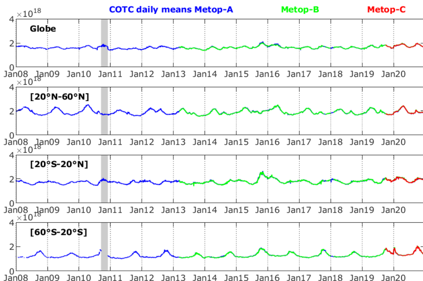
Figure 3.12. Daily (day + night) CO total columns time series (in molecules/cm 2 ), from January, 1 st 2008 until 31 December 2020, for IASI-A in blue, IASI-B in green and IASI-C in red, for the entire globe (top) and different latitude bands. The shaded grey band corresponds to the time period 14/09/2010-02/12/2010 when EUMETSAT only delivered clear sky L2 pixels (i.e. with cloud cover equal to 0): It dramatically reduced the number of FORLI-CO retrieved pixels.
