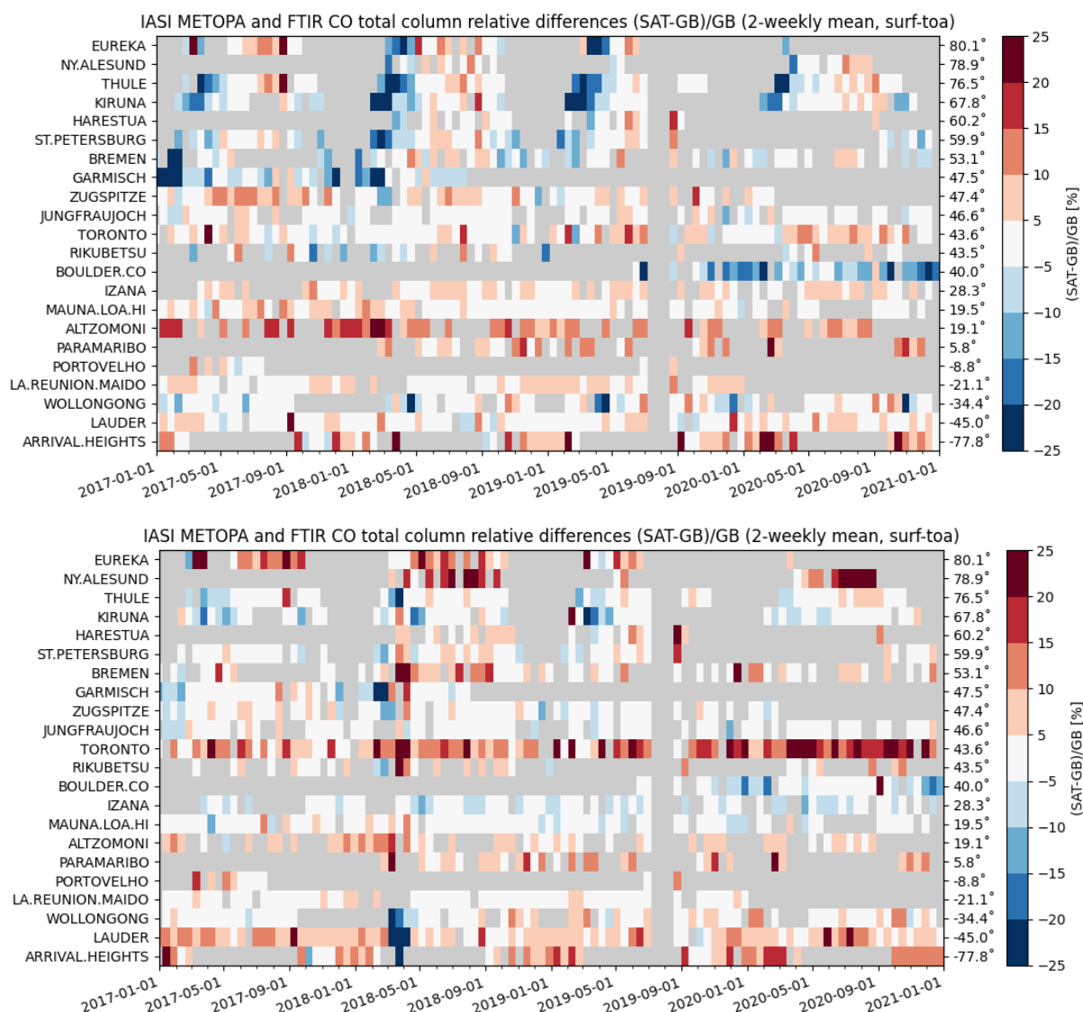
Figure 2.5. Time series of bi-weekly relative difference for IASI Metop-A against NDACC FTIR for the direct comparison (top) and the comparison with smoothing (bottom).
