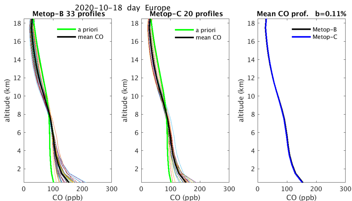
Figure 3.11. Same as Figs 3.6 to 3.10 but for 2020-10-18, over the European region.
