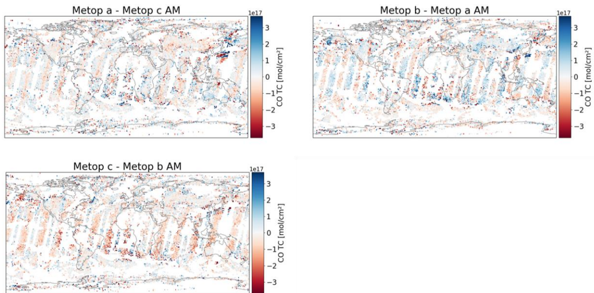
Figure 3.2. CO total column differences on a 1x1 degree grids for the observations shown in Figure 3.1
