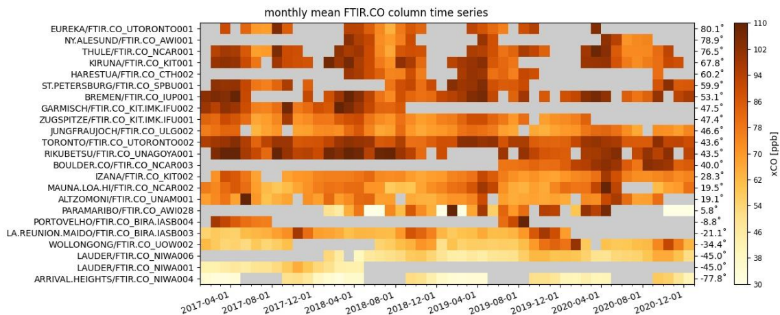
Figure 2.1 Overview of NDACC instruments with CO measurement data in 2017-2020. Time series shows column dry averaged xCO and instruments are labelled by site, institute and number (left) and are sorted by latitude (indicated on the right). FTIR measure direct sunlight and hence no measurements are available at high latitude stations during local winter.
