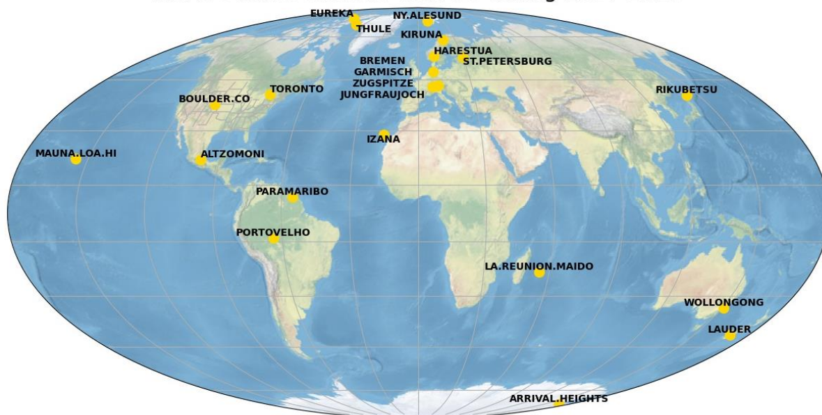
Figure 2.2 World map showing the 22 NDACC stations with CO data during the period 2017-2020.
