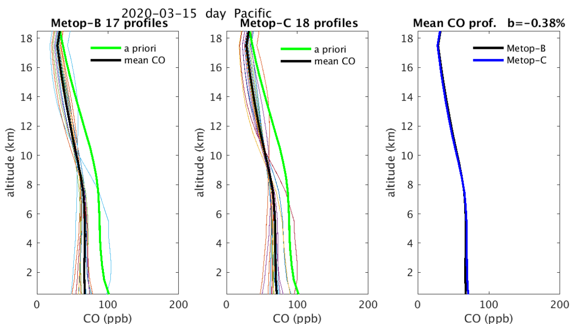
Figure 3.6. Pacific, 2020-03-15. Left: Metop-B profiles in color, mean profile in bold black and a priori profile in bold green. Middle: Same as left but for Metop-C. The two mean profiles are also in the right panel. Relative bias is indicated in the title of right panel.
