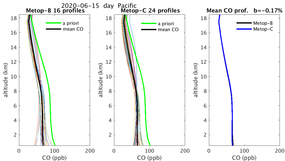
Figure 3.7. Same as Fig. 3.6 but for 2020-06-15.
