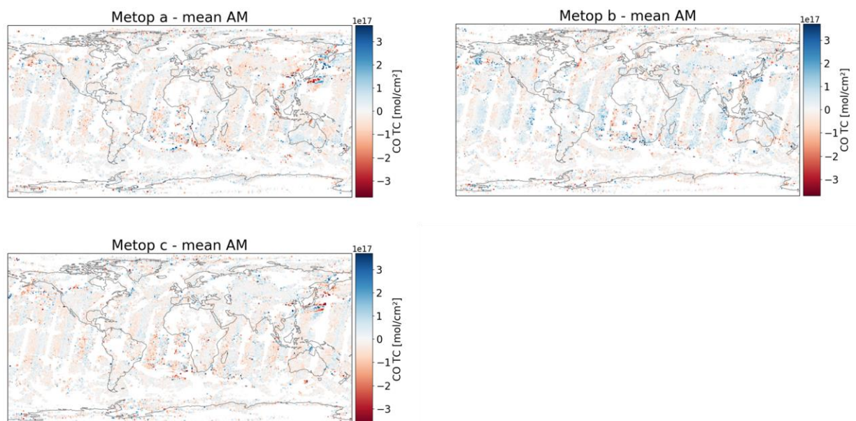
Figure 3.3. CO differences with respect to the mean of the three instruments on 1x1 grid (mean is shown in the last panel of Figure 3.1).
