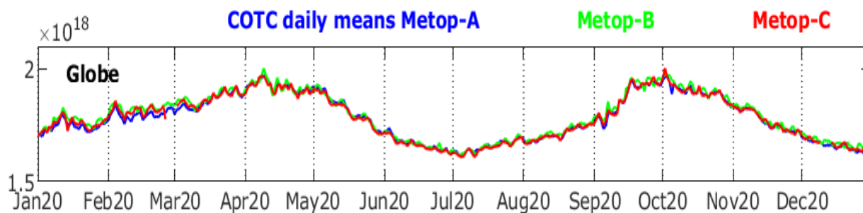
Figure 3.13. 2020 daily (day + night) CO total columns time series for IASI-A in blue, IASI-B in green and IASI-C in red, for the entire globe.
