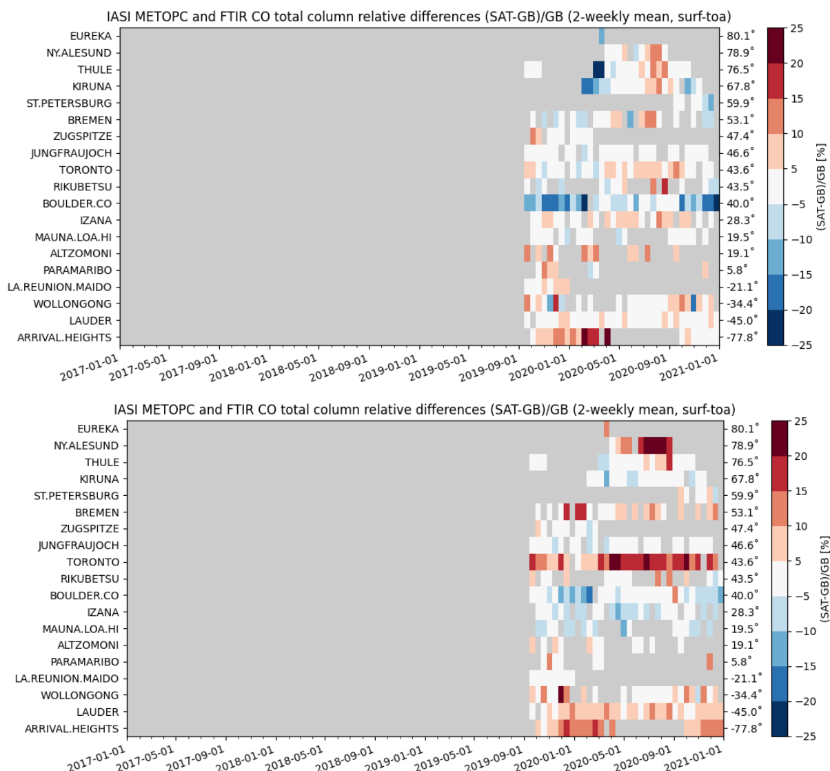
Figure 2.7. Time series of bi-weekly relative difference for IASI Metop-C against NDACC FTIR for the direct comparison (top) and the comparison with smoothing (bottom). Not all stations have co-locations with the IASI Metop-C satellite. Although the Metop-C time series is too short to deduce robust statistics, the time series of the bias corresponds closely to the Metop-A/B time series and the time series shows similar features.
