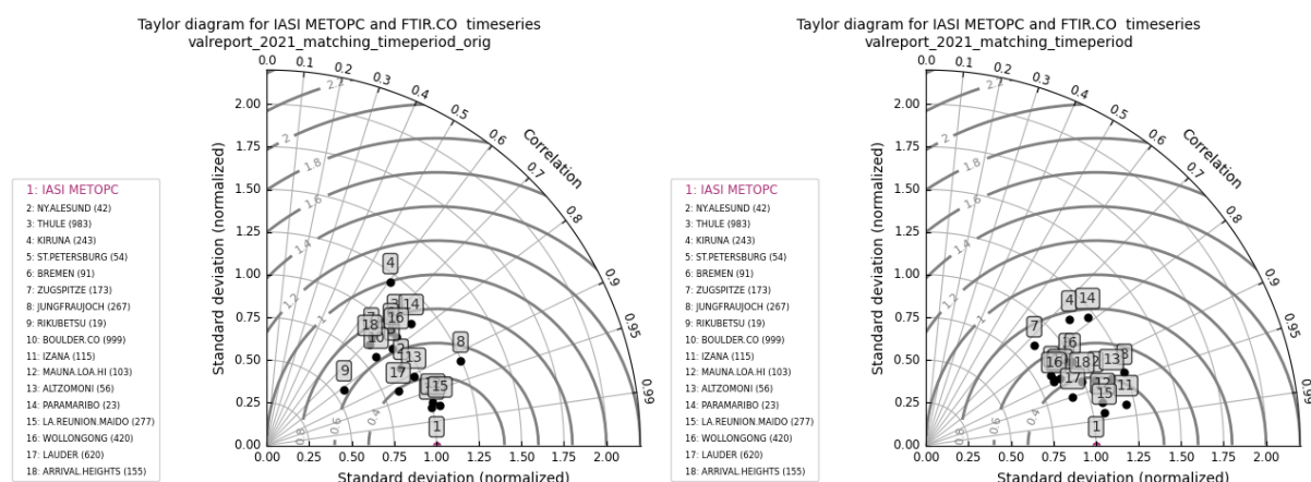
Figure 2.4. Correlation plots for IASI Metop-C direct comparison data (left) and IASI Metop-C smoothed comparison data (right). The Taylor diagram shows the impact of the smoothing operation on the statistics: most correlations shift to values above 0.8.
